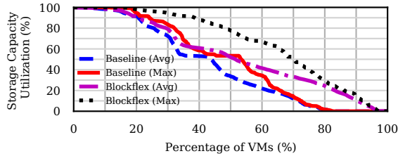
Figure 15: Improved utilization for underutilized storage.
