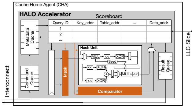
Figure 6: The architecture of HALO accelerator.
