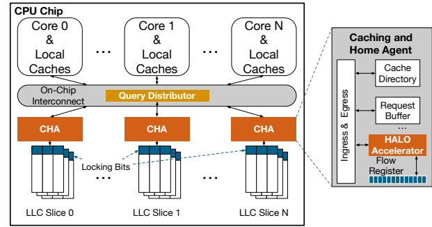
Figure 5: The overview of HALO architecture.
