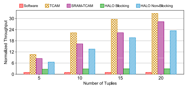
Figure 11: Performance comparison with tuple space search.
