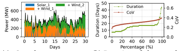
(a) Complementary power production of three sites. (b) Duration of the complementary patterns.
