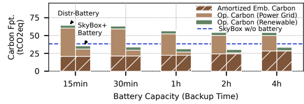
Figure 15: Total carbon footprint as we vary the battery capacity in modular data centers.
